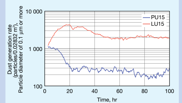
Fig. 1-2 Dust generation rate
