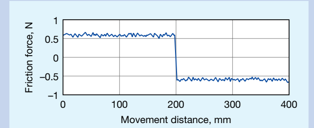
Fig. 1-1 Fluctuations in dynamic friction
